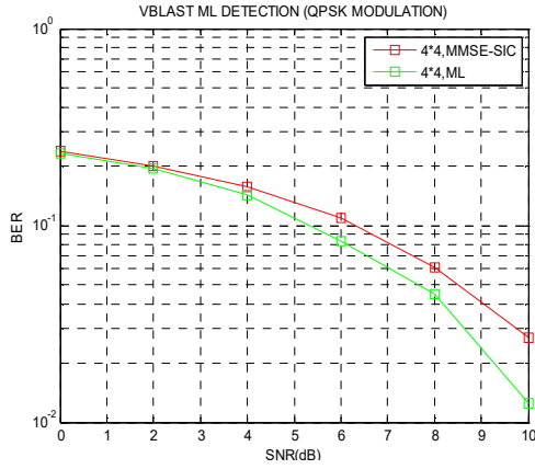
Figure 8. BER performances of V-BLAST ML detection (QPSK)
