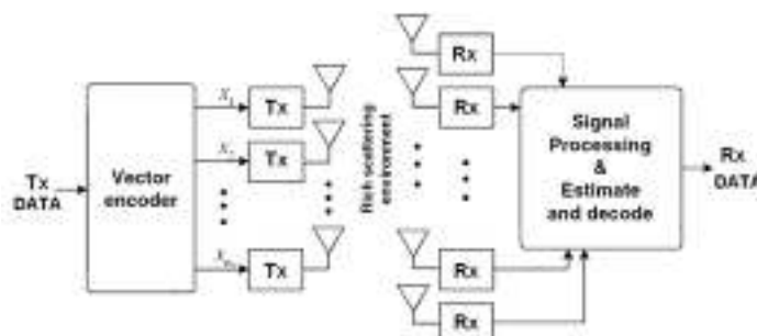
Figure 1. V-Blast system
