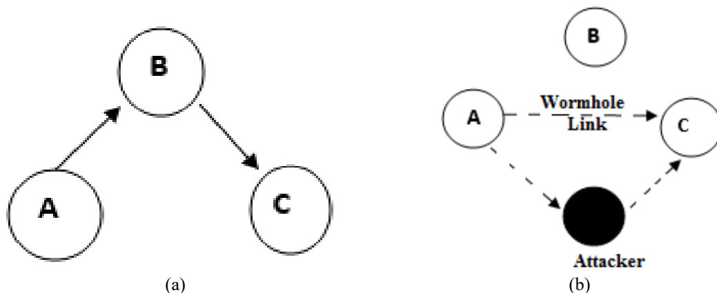
Figure 2. Wormhole attack
